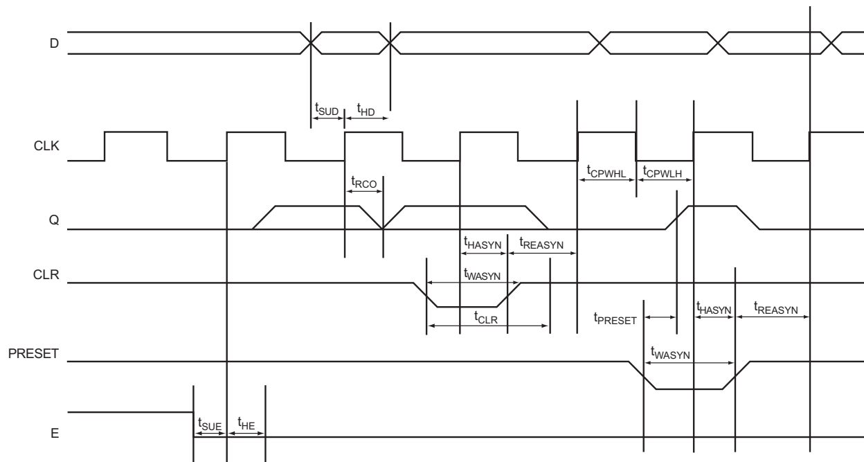
Figure 2-36 • R-Cell Delays
