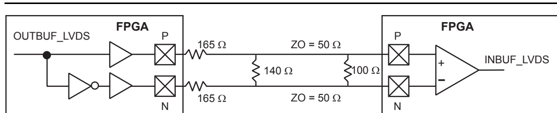
Figure 2-26 • LVDS Circuit
