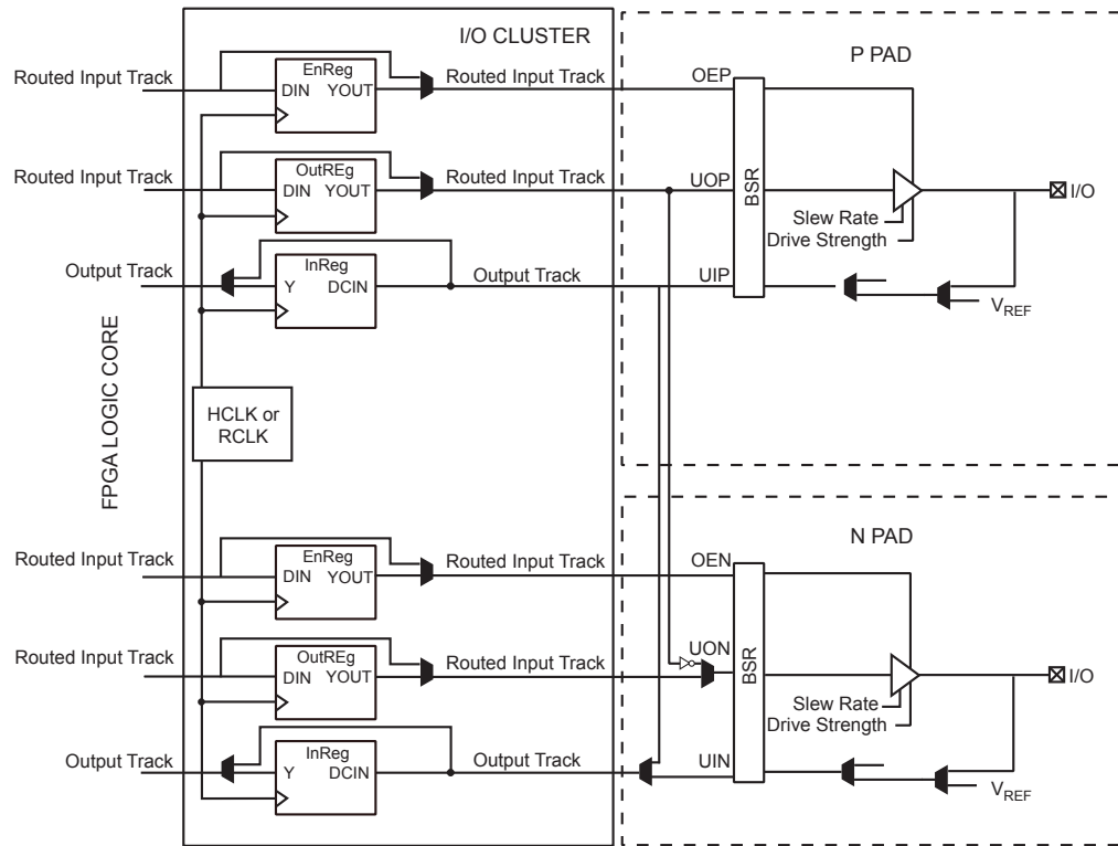
Figure 2-5 • I/O Cluster Interface
